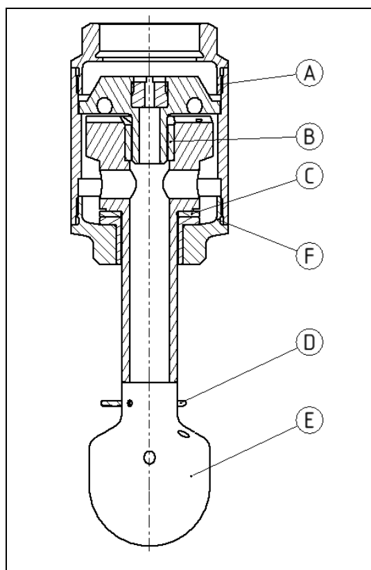
Picture 7.4-2: CP3 Maintenance Points
