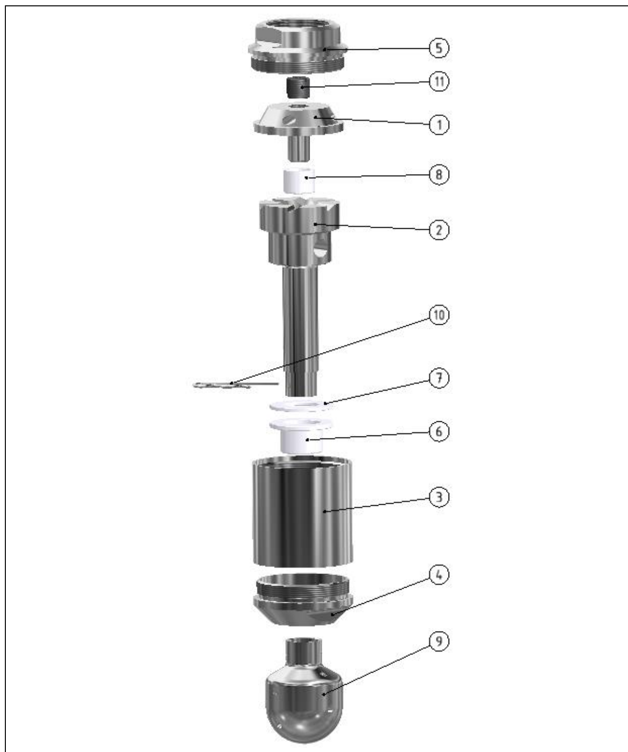
Picture 7.4-4: Exploded diagram of the CP3 device
