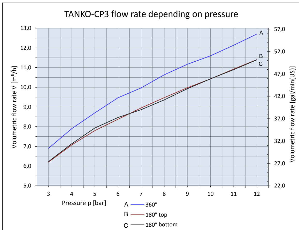
Picture 3.3-3: TANKO-CP3 consumption data
